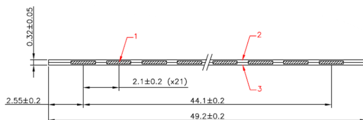
Fig. 3: Signal flat cable 20 conductors each close to AWG26
