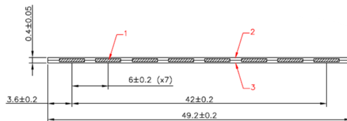
Fig. 2: Power flat cable 8 conductors each close to AWG18
