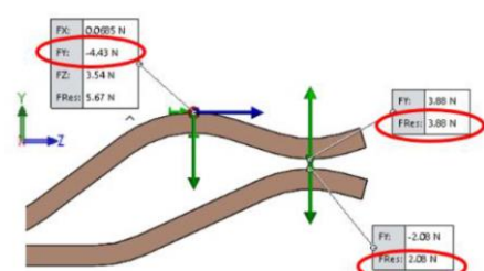
Fig. 5: Calculation of forces and optimisation of the shape, thickness and material state of the contact.
