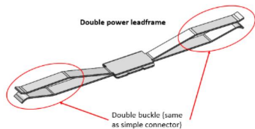
Fig. 25: Power contact for panel feedthrough connector variant.
